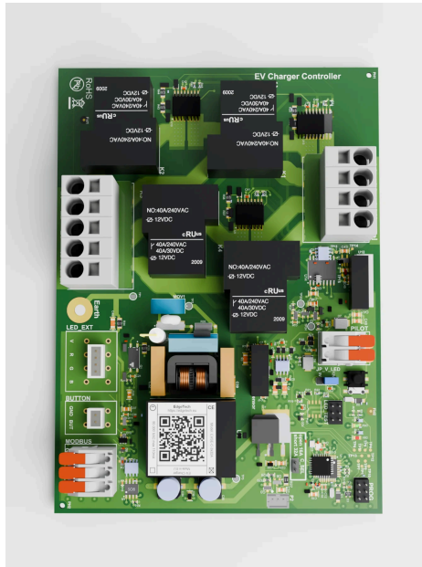
The charge controller board, 168 × 122 mm
